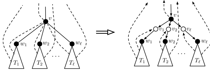
Figure 2: The gadget that, for each child of v , introduces a new vertex (depicted in white) and redirects back-arcs.
