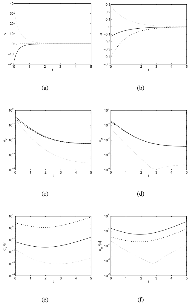
Fig. 6. PBVS behavior in world frame: Velocity (a) translation; (b) rotation; Absolute errors (c) translation; (d) rotation; Relative errors (e) translation; (f) rotation.
