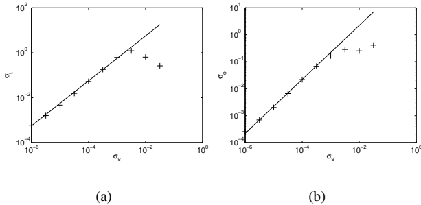
Fig. 2. Measured and predicted deviations in pose estimates with respect to image error: (a) translation; (b) rotation angle.
