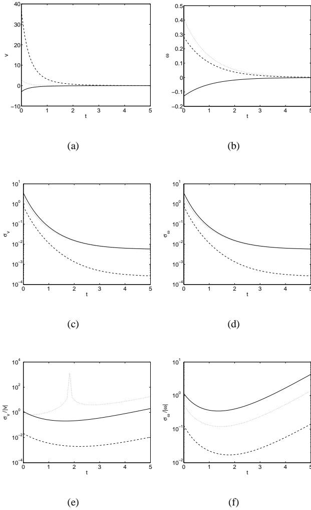
Fig. 10. HYBVS behavior in camera frame: Velocity (a) translation; (b) rotation; Absolute errors (c) translation; (d) rotation; Relative errors (e) translation; (f) rotation.
