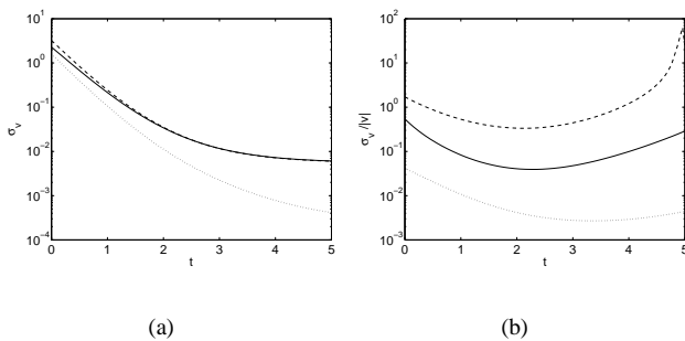
Fig. 11. HYBVS translation errors on PBVS trajectory: (a) absolute; (b) relative.
