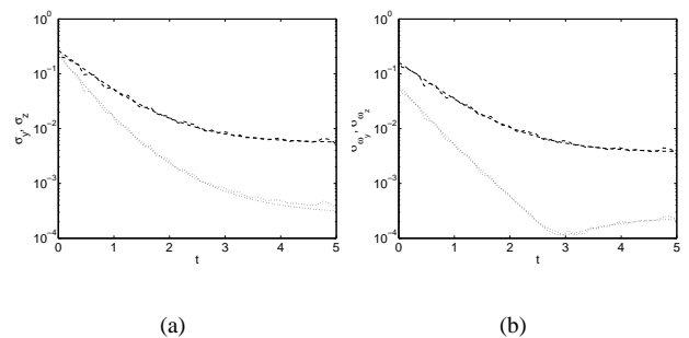
Fig. 5. Measured and predicted deviations in PBVS control output: (a) translation; (b) rotation.
