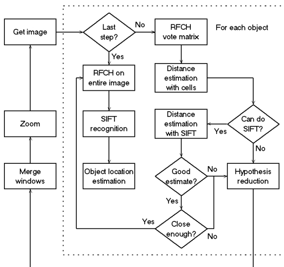
Figure 3: Object search algorithm.
