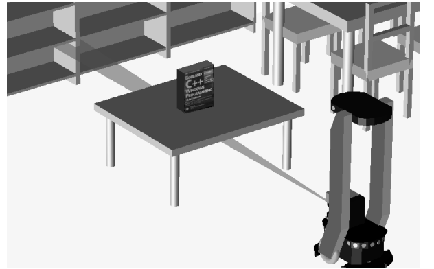
Figure 5: Distance estimation provided by the laser may not be reliable: instead of the distance to the object on the table, the distance to the shelf is measured.
