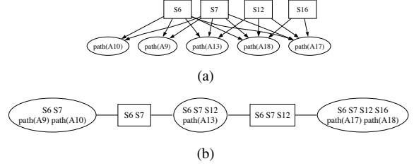
Figure 5. Bayesian network (a) and junction tree (b) for the track graph in Figure 2
