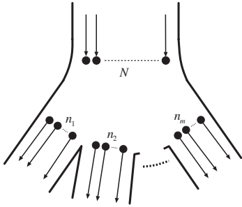
Figure 3. The size of the state variable of a split node is determined by the number of outgoing tracks and how many targets, n_i are in each track i .
