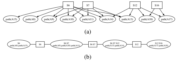
Figure 6. To reduce the complexity we remove dependencies between tracks that are distant in time. The result is that the algorithm optimizes shorter local paths that are overlapping. The Bayesian network (a) now has paths to all single track nodes with ancestors and A_{17} and A_{18} does not depend on S_6 and S_7 anymore. (b) shows the resulting junction tree.
